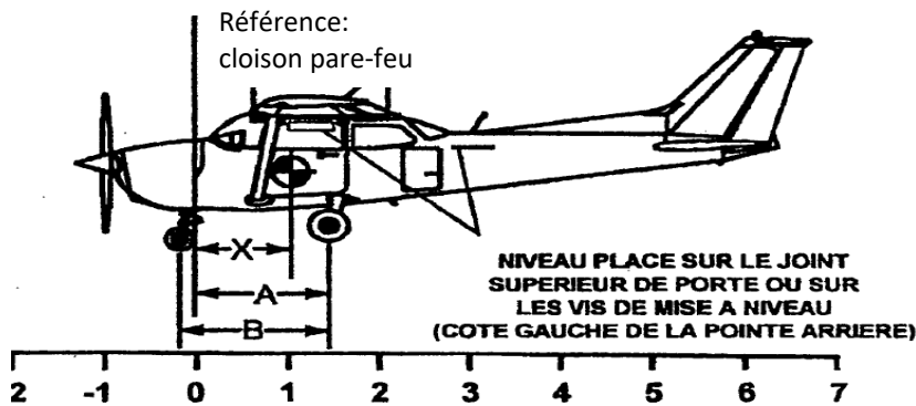
STATIONS DE FUSELAGE (STA) - m
